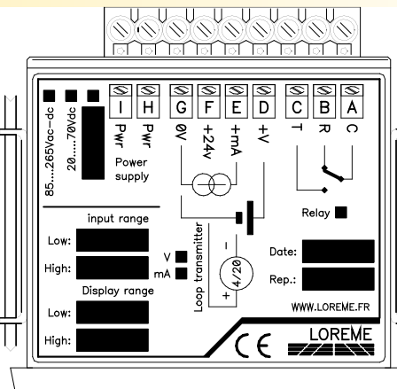
4..20mA / 0...10V input version
